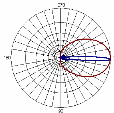
2 degree down tilt shown
